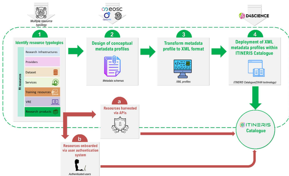
Figure 1 Workflow for the design and implementation of the ITINERIS metadata catalogue
