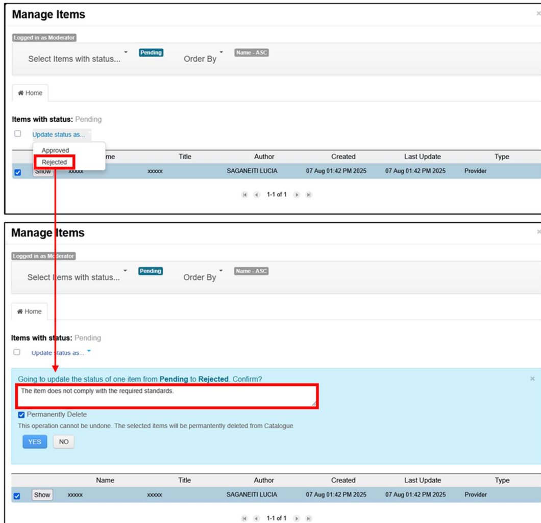
Figure 7 Permanently delete item example
